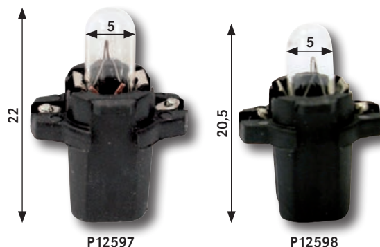
P12597
