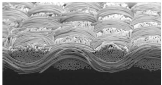
Photos are Scanning Electron Microscope (SEM) >300X magnification showing front and side views of a typical 1000D air textured Nylon CORDURA® fabric
